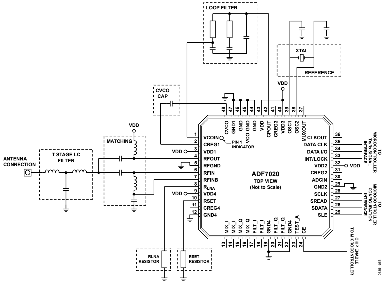
Figure 41. Application Circuit
