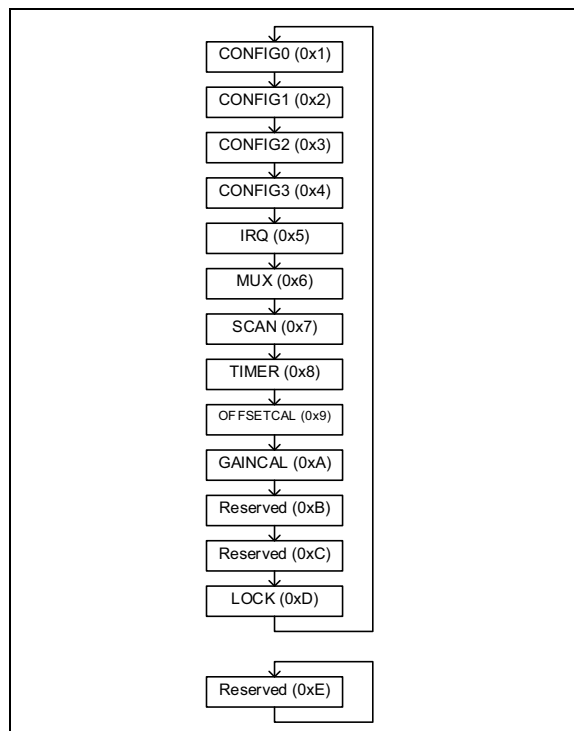
FIGURE 6-3: Incremental Write Loop.
