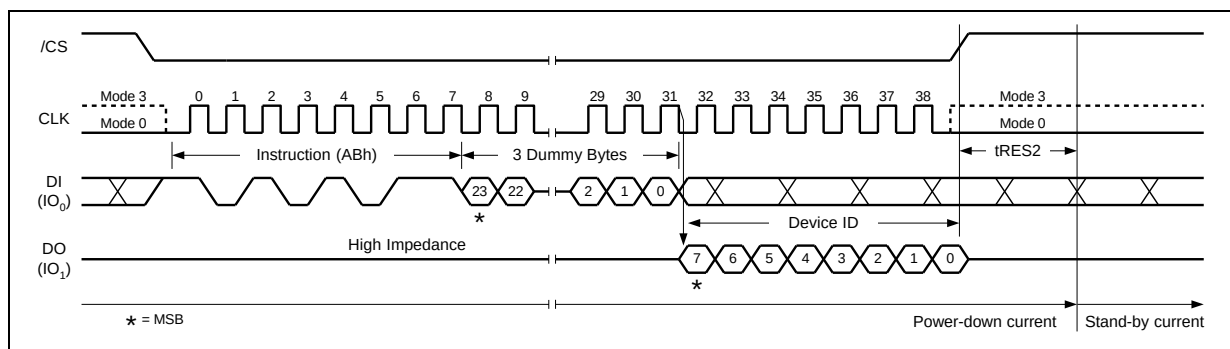
Figure 38c. Release Power-down / Device ID Instruction
