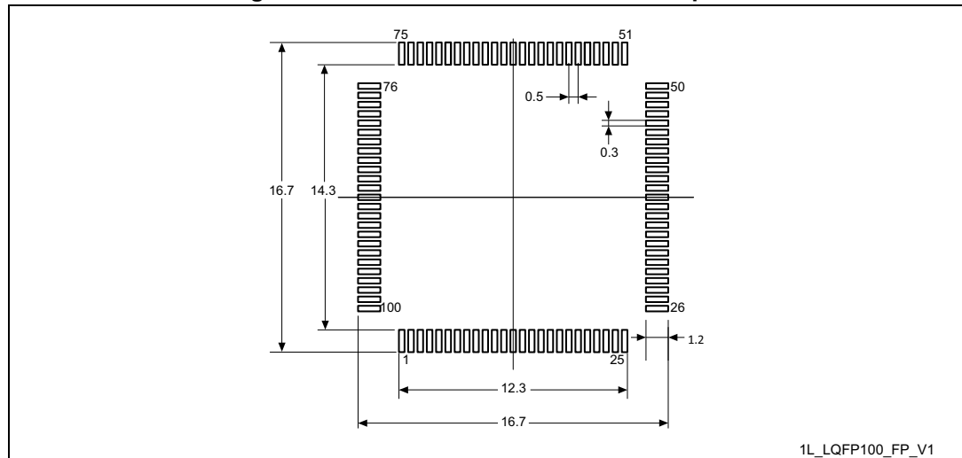
Figure 80. LQFP100 - Recommended footprint
